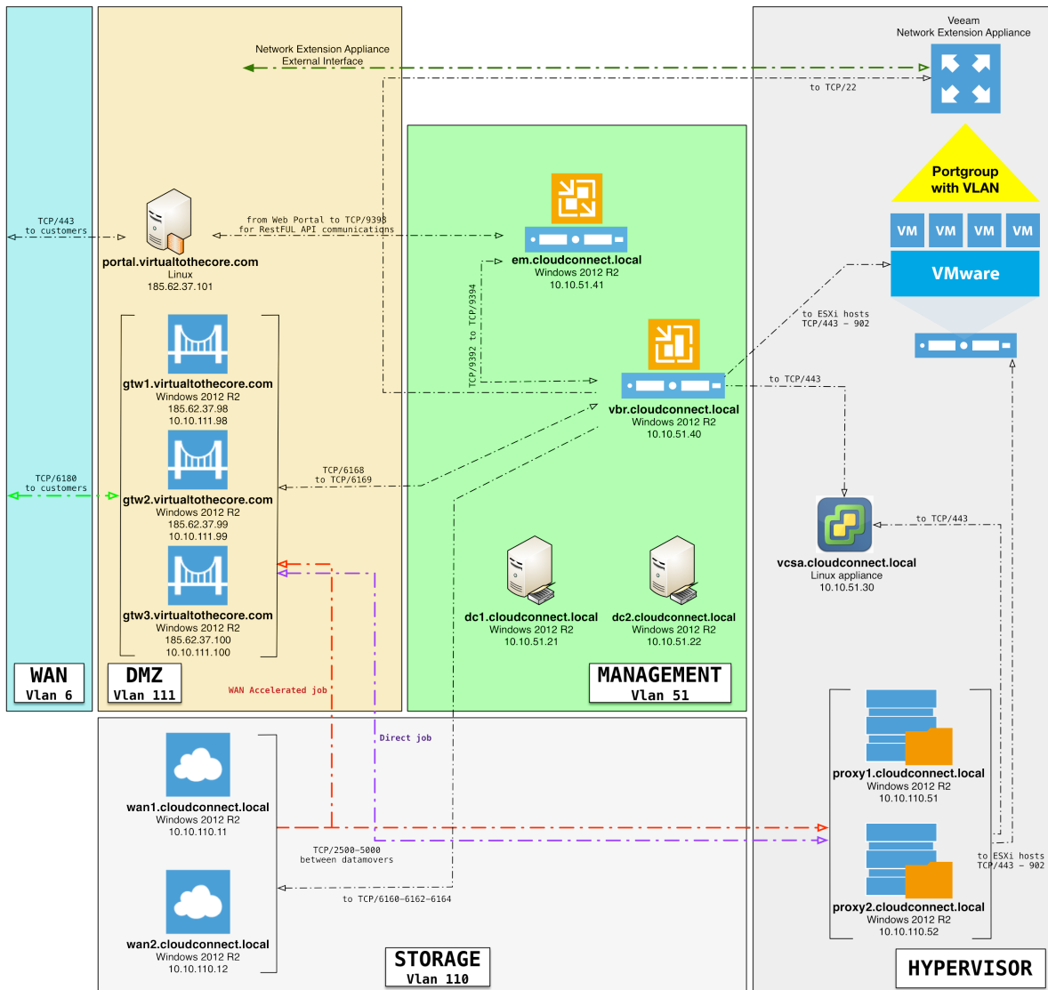
4.11: Veeam Cloud Connect Replication servers diagram
