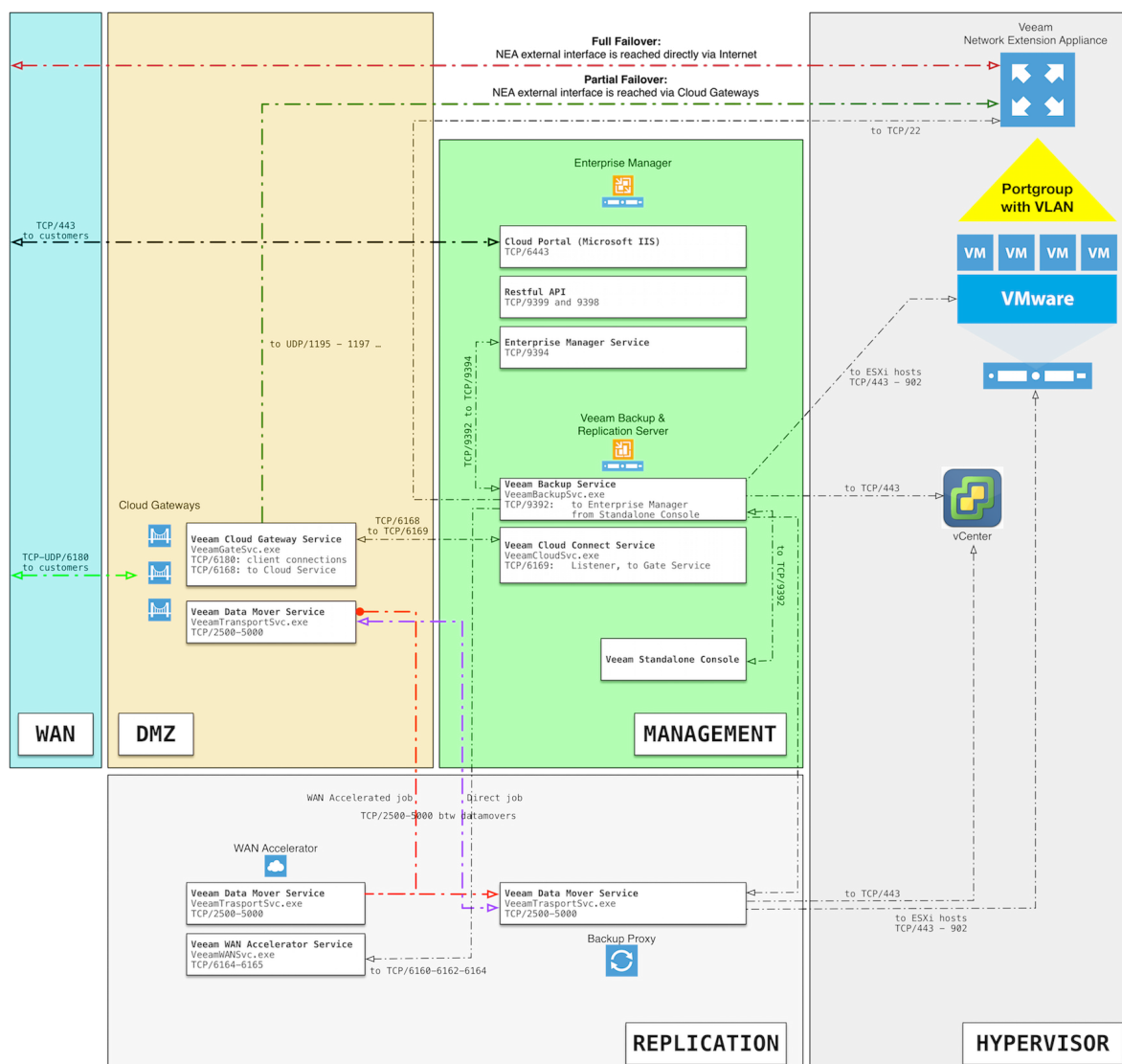
4.10: Veeam Cloud Connect Replication diagram
