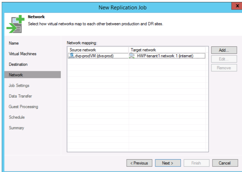
5.41: Network mapping
